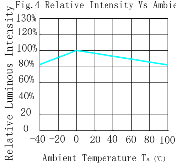
Fig.4 Relative Intensity Vs Ambient Temperature
